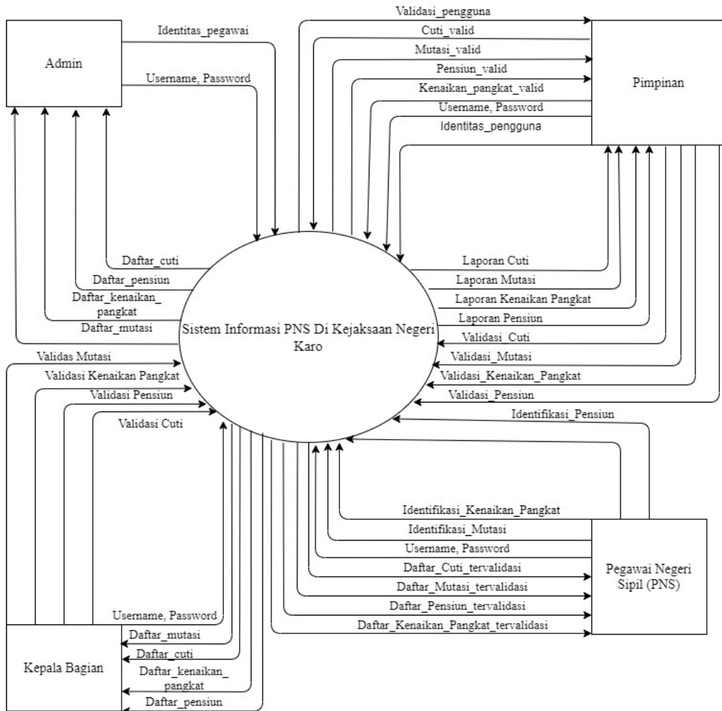
Gambar 3.5 Diagram Konteks
